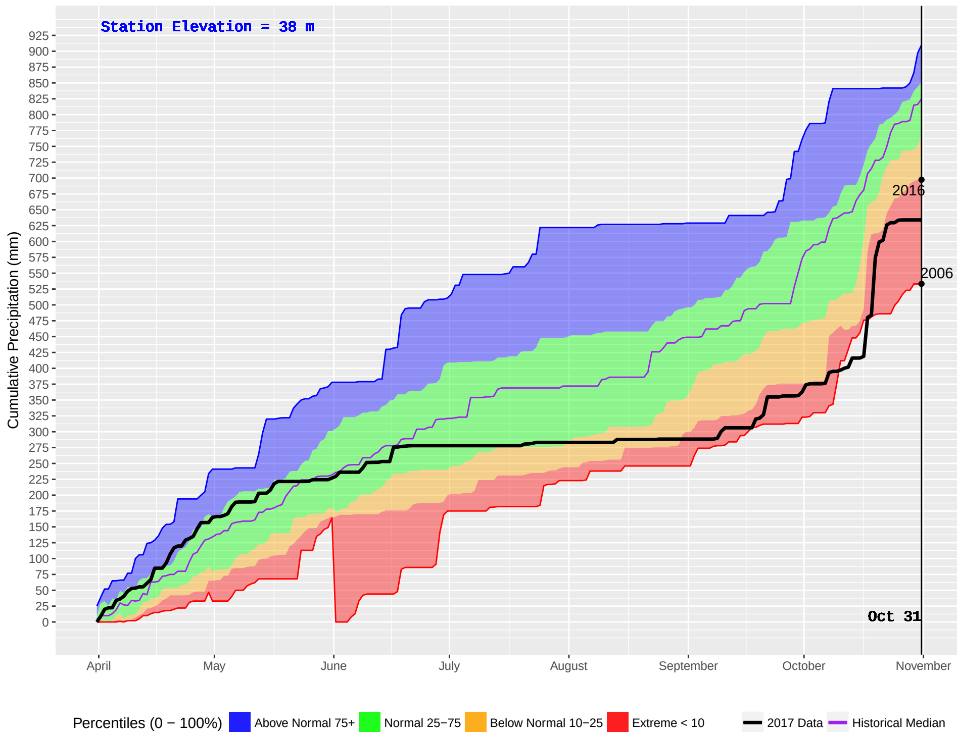
HAIG CAMP (67) : Historical (2002–2016) and Current (2017) Noon Cumulative Precipitation
