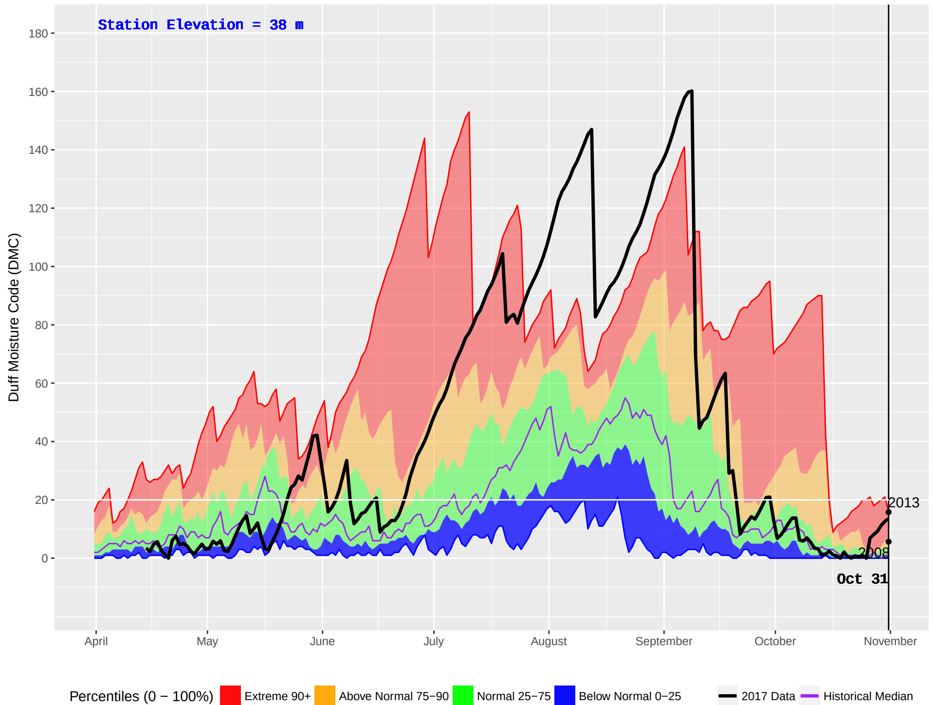
HAIG CAMP (67) : Historical (2002–2016) and Current (2017) Noon Duff Moisture Code (DMC)
