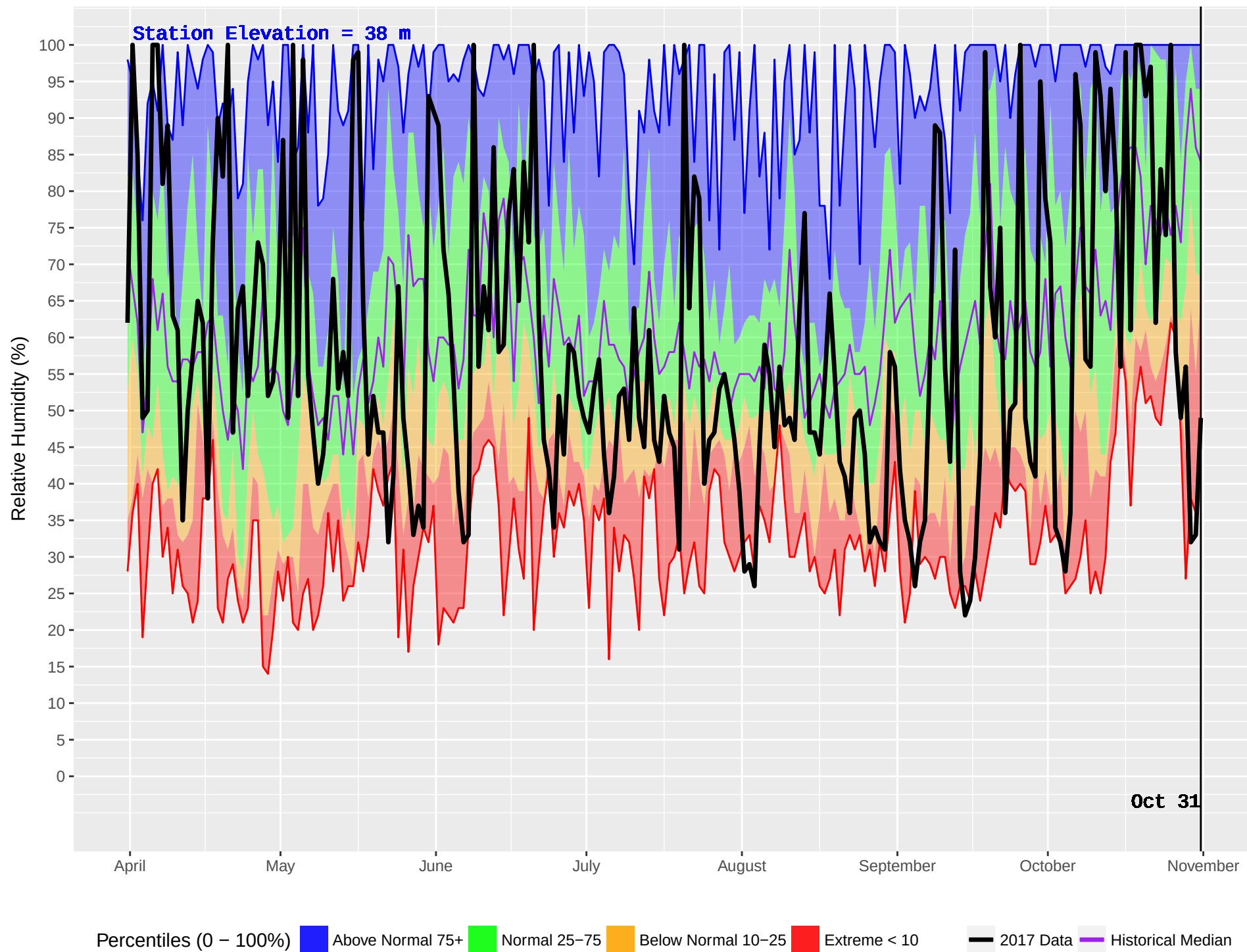
HAIG CAMP (67) : Historical (2002–2016) and Current (2017) Noon Relative Humidity
