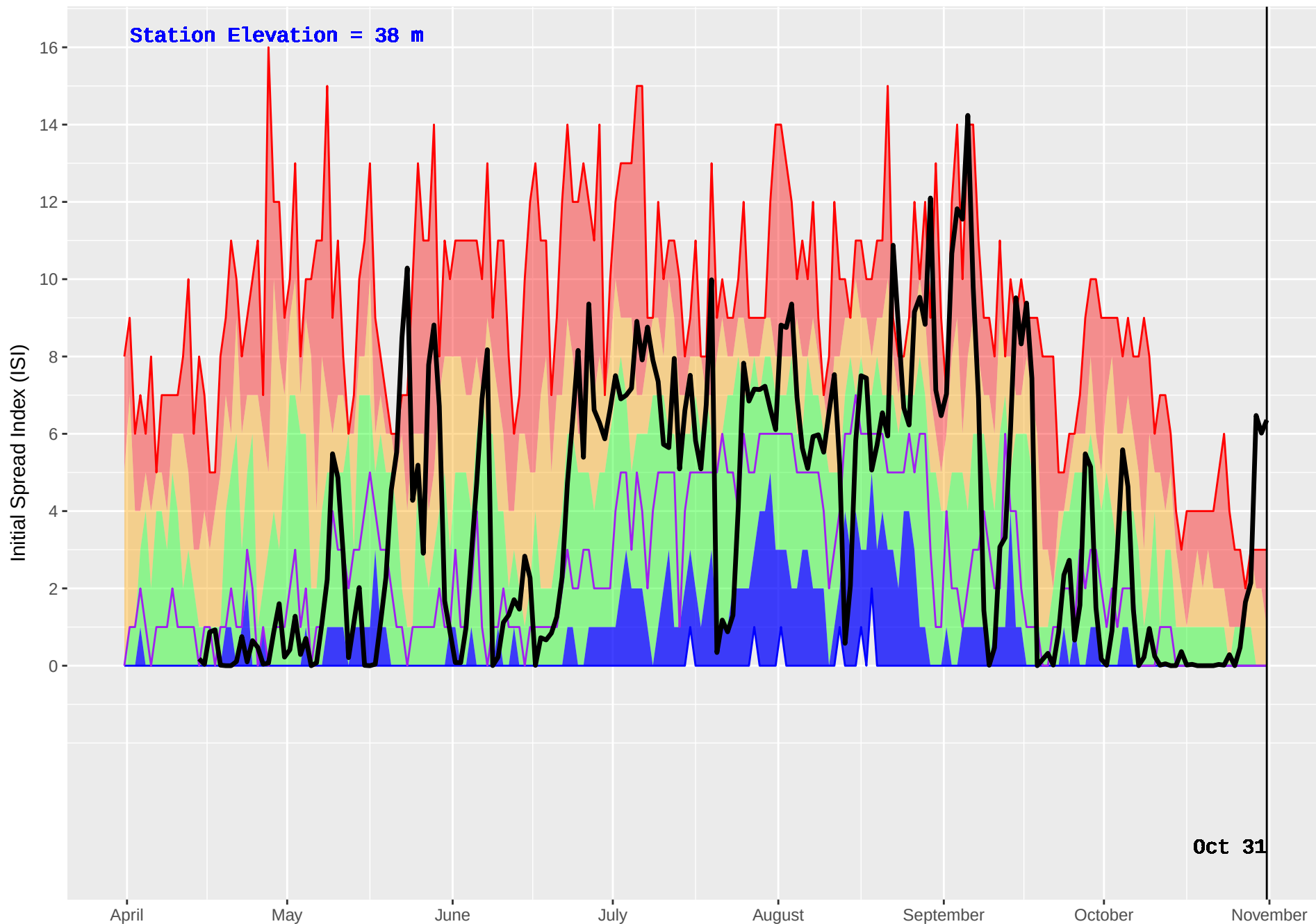
HAIG CAMP (67) : Historical (2002–2016) and Current (2017) Noon Initial Spread Index (ISI)
